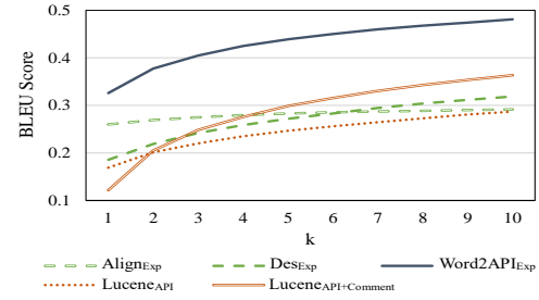
Fig. 6: BLEU score for different expansion algorithms.
