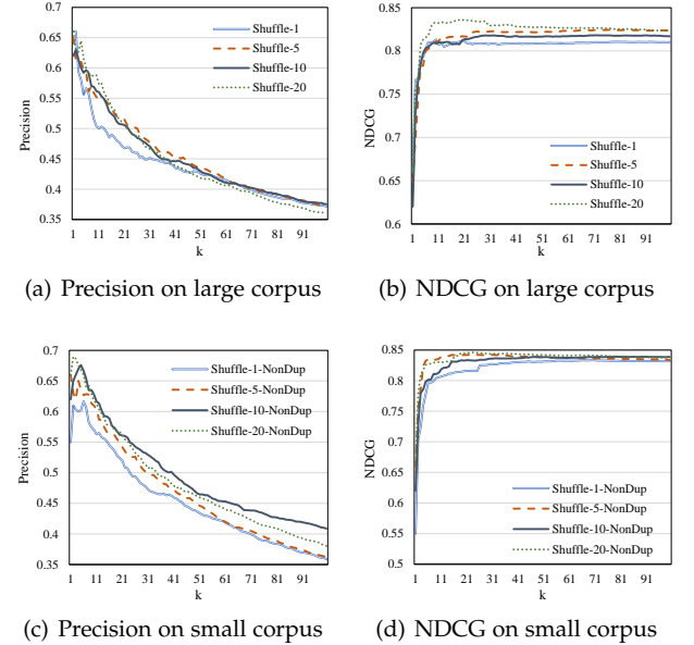
Fig. 2: Influence on shuffling times.
