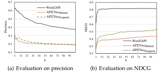
Fig. 1: Comparison with API2Vec.
