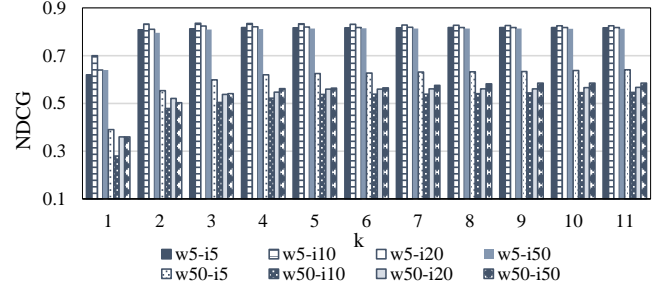
(b) NDCG on the number of iterations
