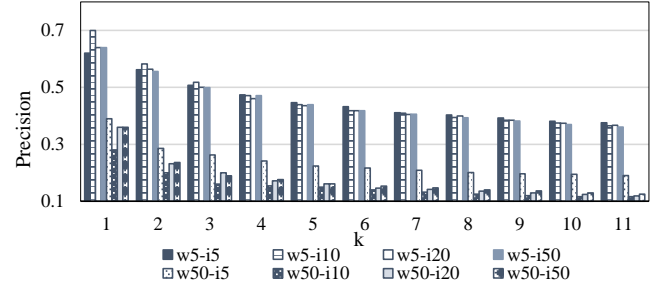
(a) Precision on the number of iterations
